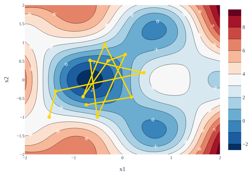
Gradient Descent Path from (-1.5, -1) , Step Size = 0.25
