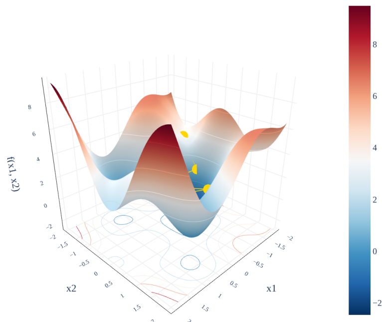
Gradient Descent Path from (-1.5, -1) , Step Size = 0.25
