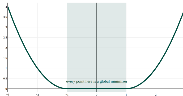
A convex function can have a flat bottom
