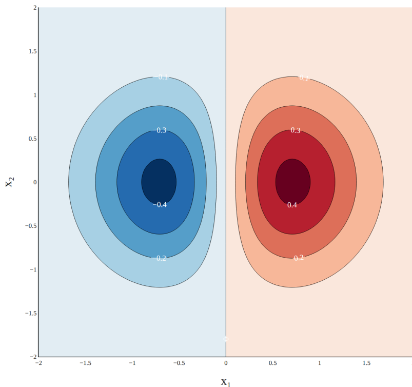
Contour plot of f(\vec{x}) = x_1 e^{-x_1^2 - x_2^2}
