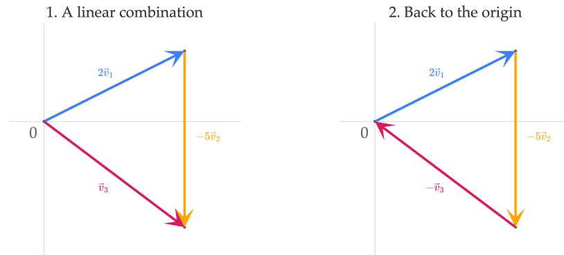
Figure 4.1: Here, \vec{v}_1 = \begin{bmatrix} 2 \\ 1 \end{bmatrix} , \vec{v}_2 = \begin{bmatrix} 0 \\ 1 \end{bmatrix} , and \vec{v}_3 = \begin{bmatrix} 4 \\ -3 \end{bmatrix} . There are two perspectives on this picture: (1) \vec{v}_3 = 2\vec{v}_1 - 5\vec{v}_2 , so \vec{v}_3 is a linear combination of \vec{v}_1 and \vec{v}_2 . (2) 2\vec{v}_1 - 5\vec{v}_2 - \vec{v}_3 = \vec{0} : following the arrows tip to tail takes us back to where we started.
