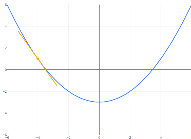
Tangent line at x = -4
